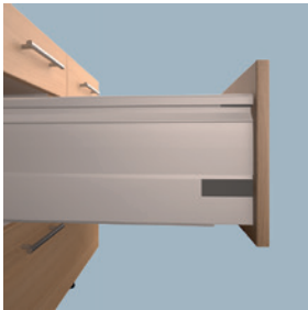
BLUM® METAL SIDED PAN DRAWER
